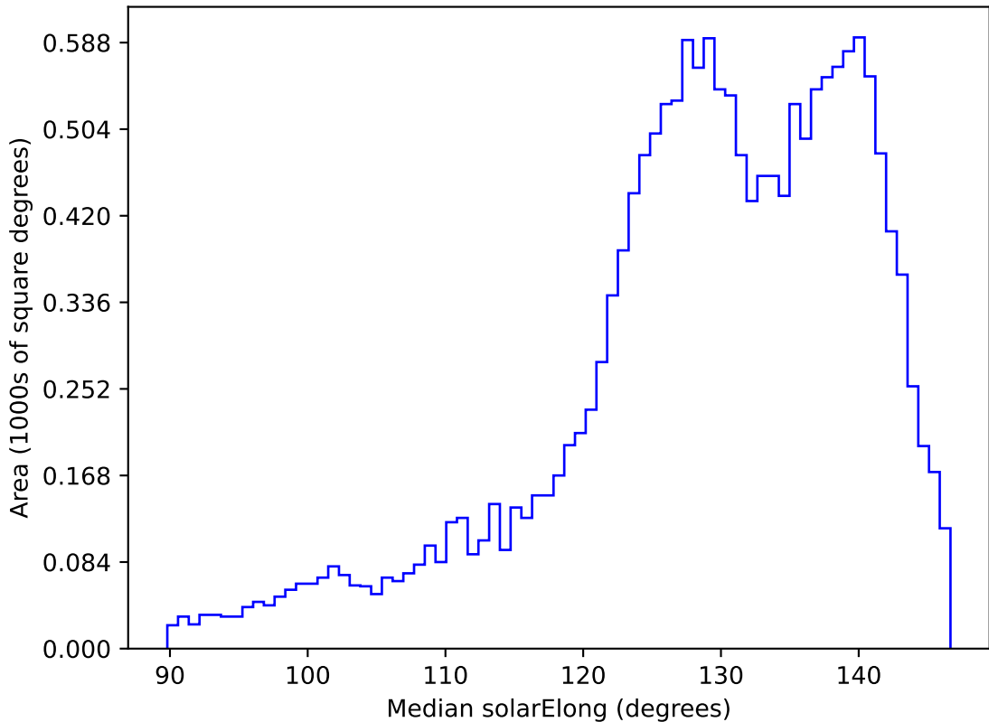
ddf_acor_sf30_lsf40_lsr20_v3.4_10yrs WFD i band: Median solarElong
