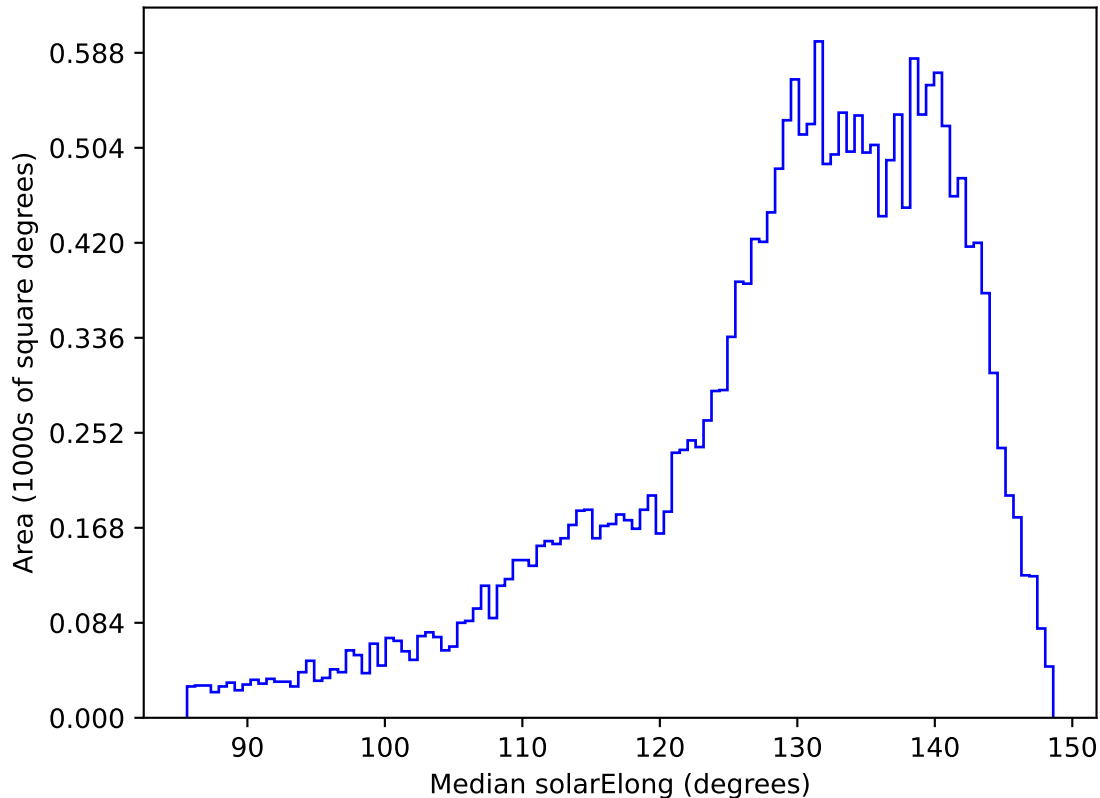
ddf_acor_sf30_lsf40_lsr20_v3.4_10yrs All sky y band: Median solarElong
