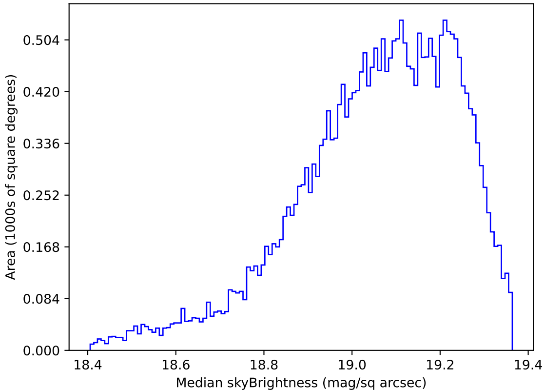
ddf_acor_sf30_lsf40_lsr20_v3.4_10yrs Yr 1 z band: Median skyBrightness
