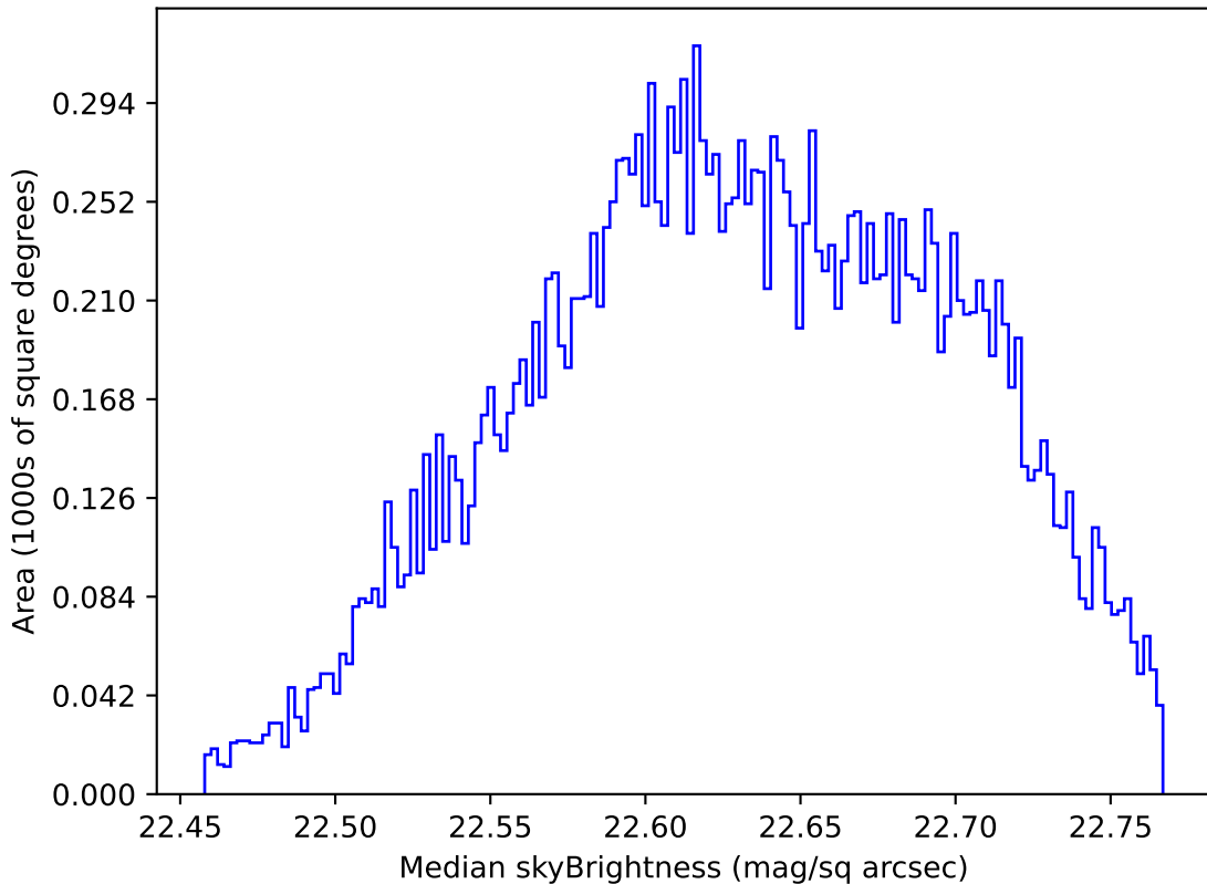
ddf_acor_sf30_Isf40_Isr20_v3.4_10yrs Yr 1 u band: Median skyBrightness
