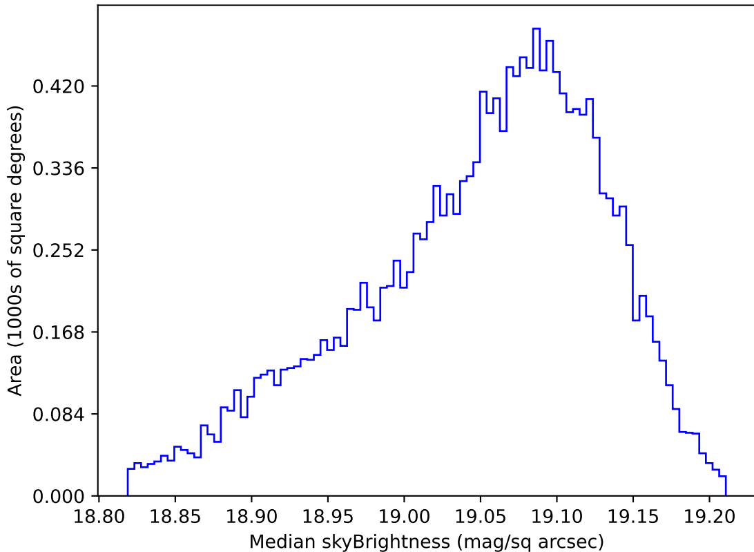
ddf_acor_sf30_lsf40_lsr20_v3.4_10yrs WFD z band: Median skyBrightness
