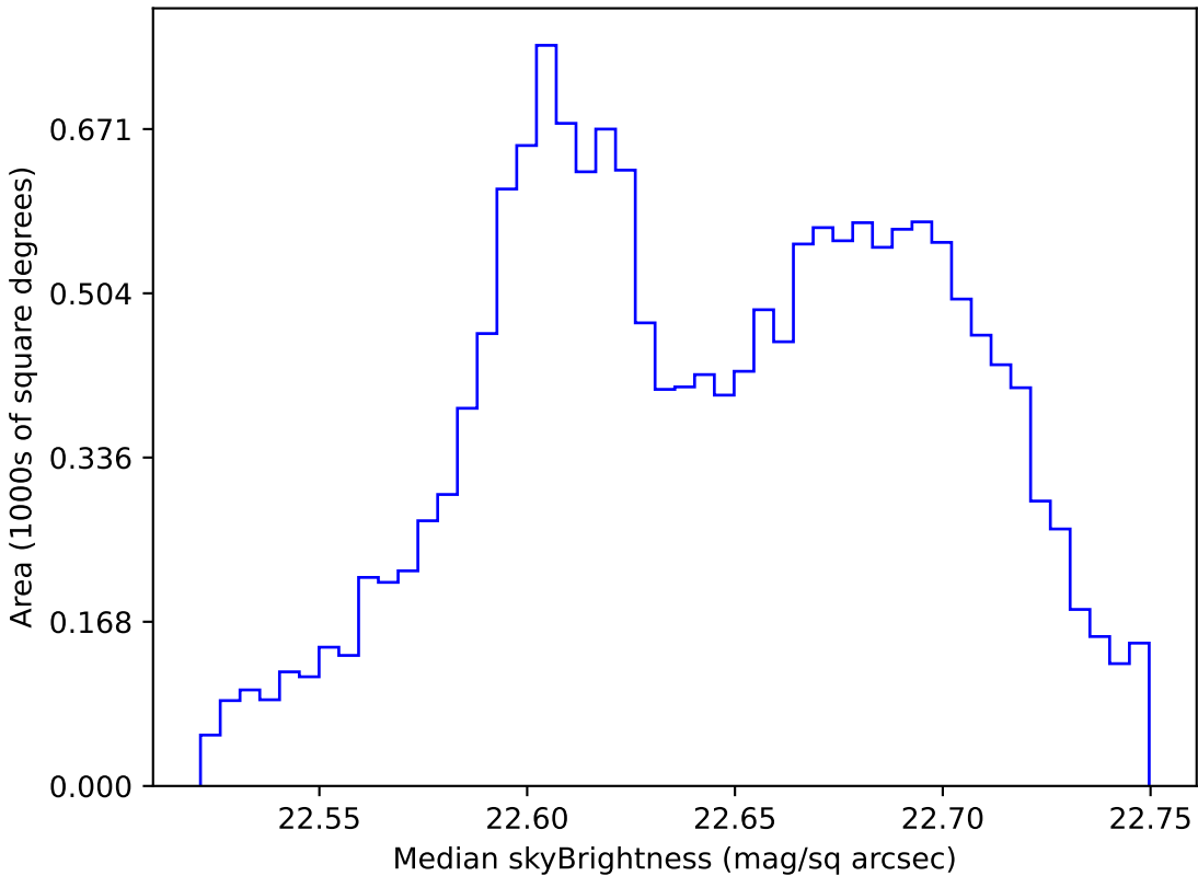
ddf_acor_sf30_lsf40_lsr20_v3.4_10yrs WFD u band: Median skyBrightness
