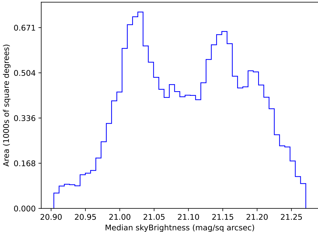
ddf_acor_sf30_lsf40_lsr20_v3.4_10yrs WFD r band: Median skyBrightness
