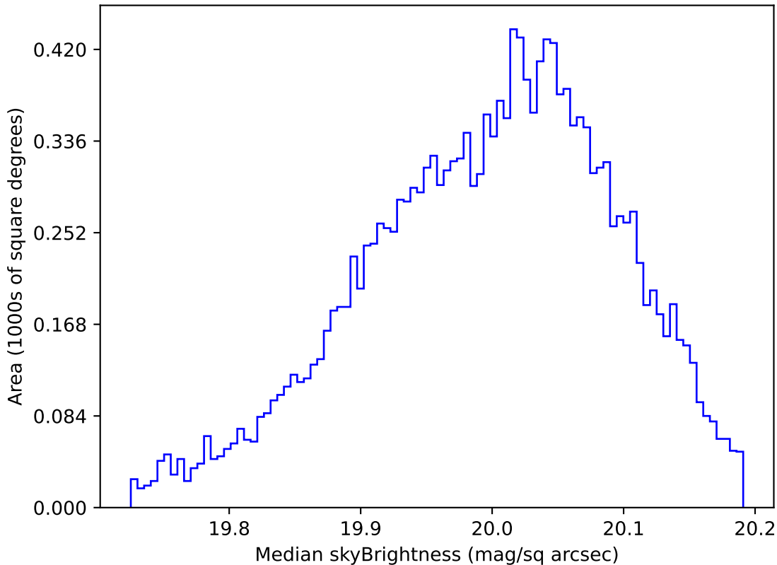
ddf_acor_sf30_lsf40_lsr20_v3.4_10yrs WFD i band: Median skyBrightness
