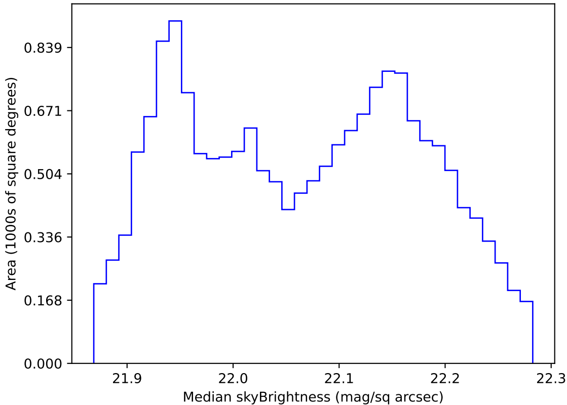
ddf_acor_sf30_lsf40_lsr20_v3.4_10yrs WFD g band: Median skyBrightness
