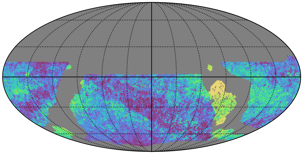
ddf_acor_sf30_lsf40_lsr20_v3.4_10yrs WFD all bands: Median skyBrightness
