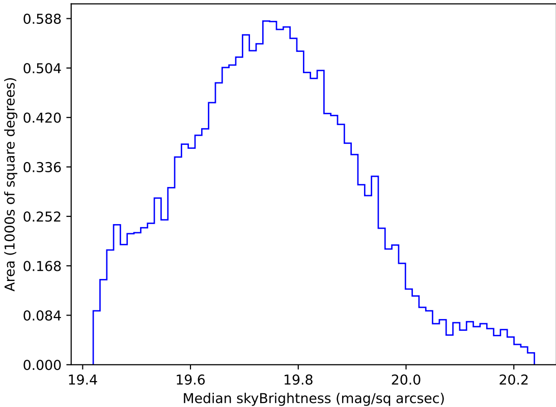
ddf_acor_sf30_lsf40_lsr20_v3.4_10yrs WFD all bands: Median skyBrightness
