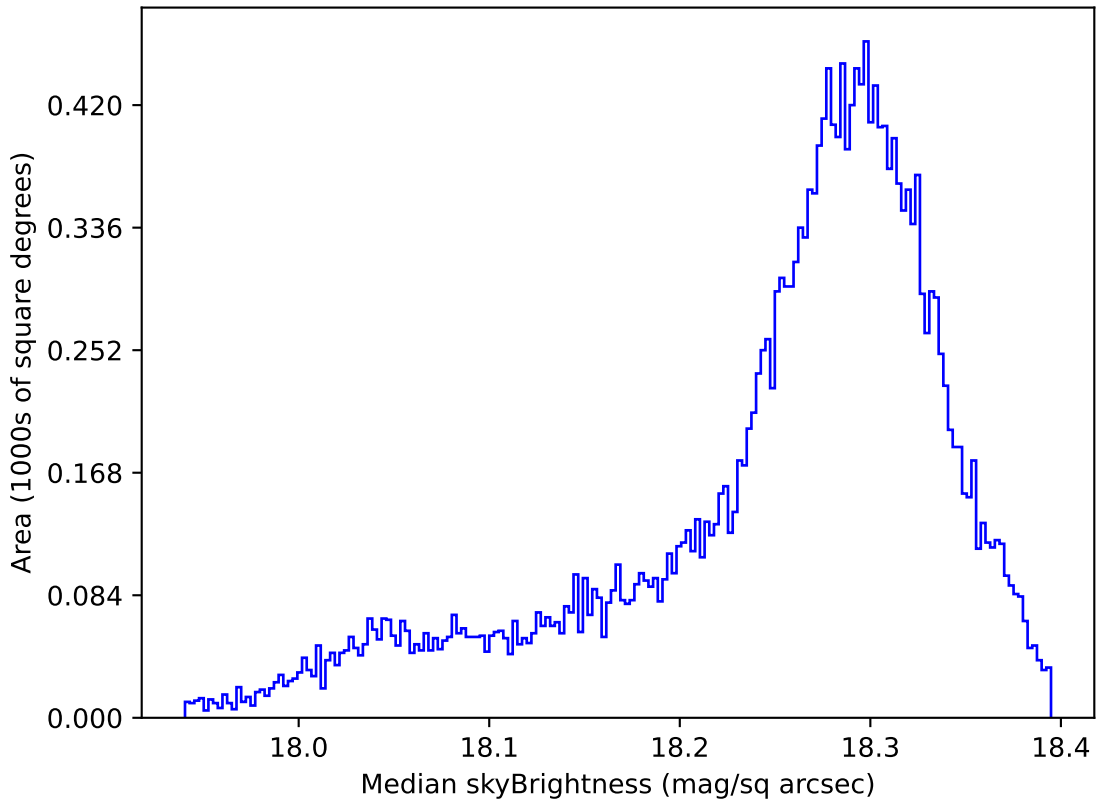
ddf_acor_sf30_lsf40_lsr20_v3.4_10yrs All sky y band: Median skyBrightness
