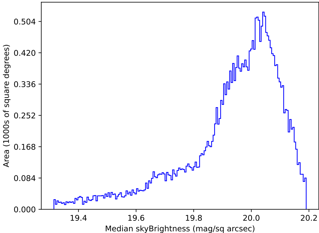
ddf_acor_sf30_lsf40_lsr20_v3.4_10yrs All sky i band: Median skyBrightness
