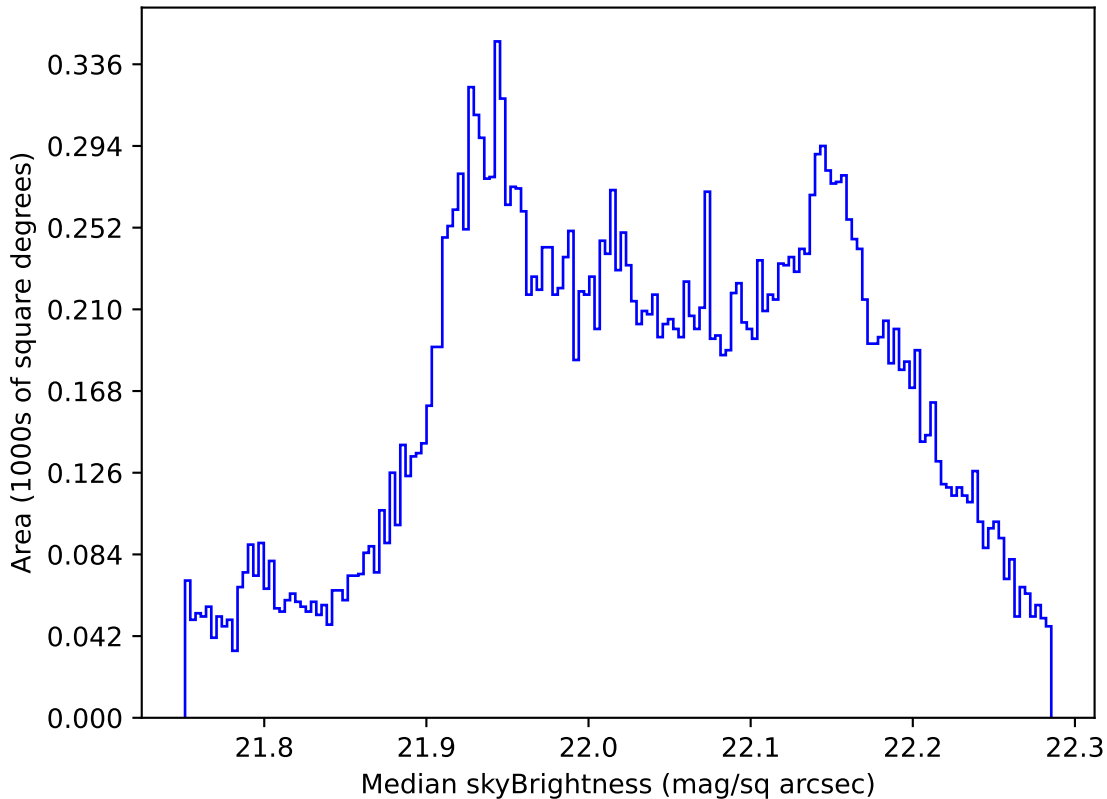
ddf_acor_sf30_lsf40_lsr20_v3.4_10yrs All sky g band: Median skyBrightness
