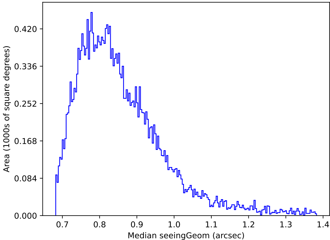
ddf_acor_sf30_lsf40_lsr20_v3.4_10yrs Yr 1 z band: Median seeingGeom
