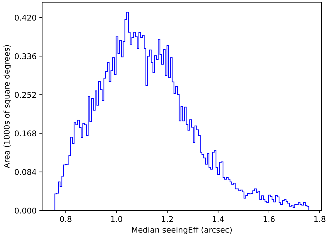
ddf_acor_sf30_lsf40_lsr20_v3.4_10yrs Yr 1 u band: Median seeingEff
