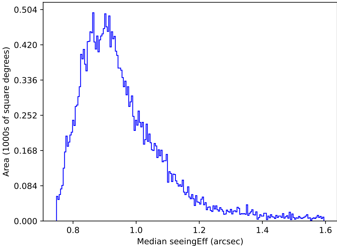
ddf_acor_sf30_lsf40_lsr20_v3.4_10yrs Yr 1 i band: Median seeingEff
