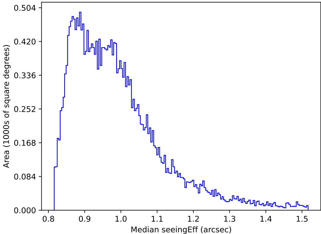
ddf_acor_sf30_lsf40_lsr20_v3.4_10yrs Yr 1 all bands: Median seeingEff
