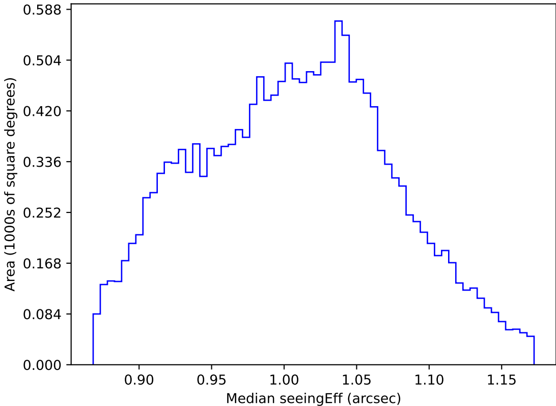
ddf_acor_sf30_lsf40_lsr20_v3.4_10yrs WFD z band: Median seeingEff
