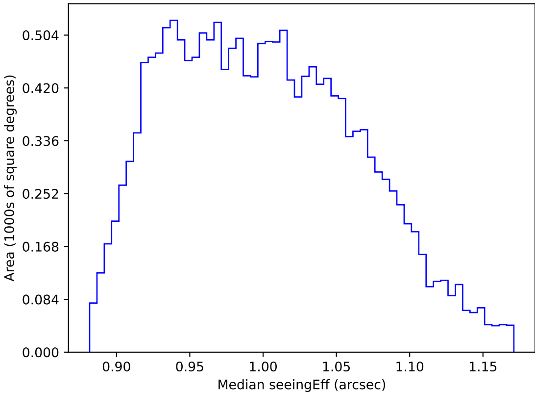
ddf_acor_sf30_lsf40_lsr20_v3.4_10yrs WFD y band: Median seeingEff
