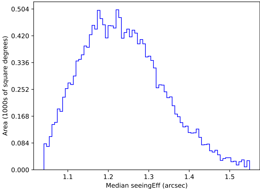
ddf_acor_sf30_lsf40_lsr20_v3.4_10yrs WFD u band: Median seeingEff
