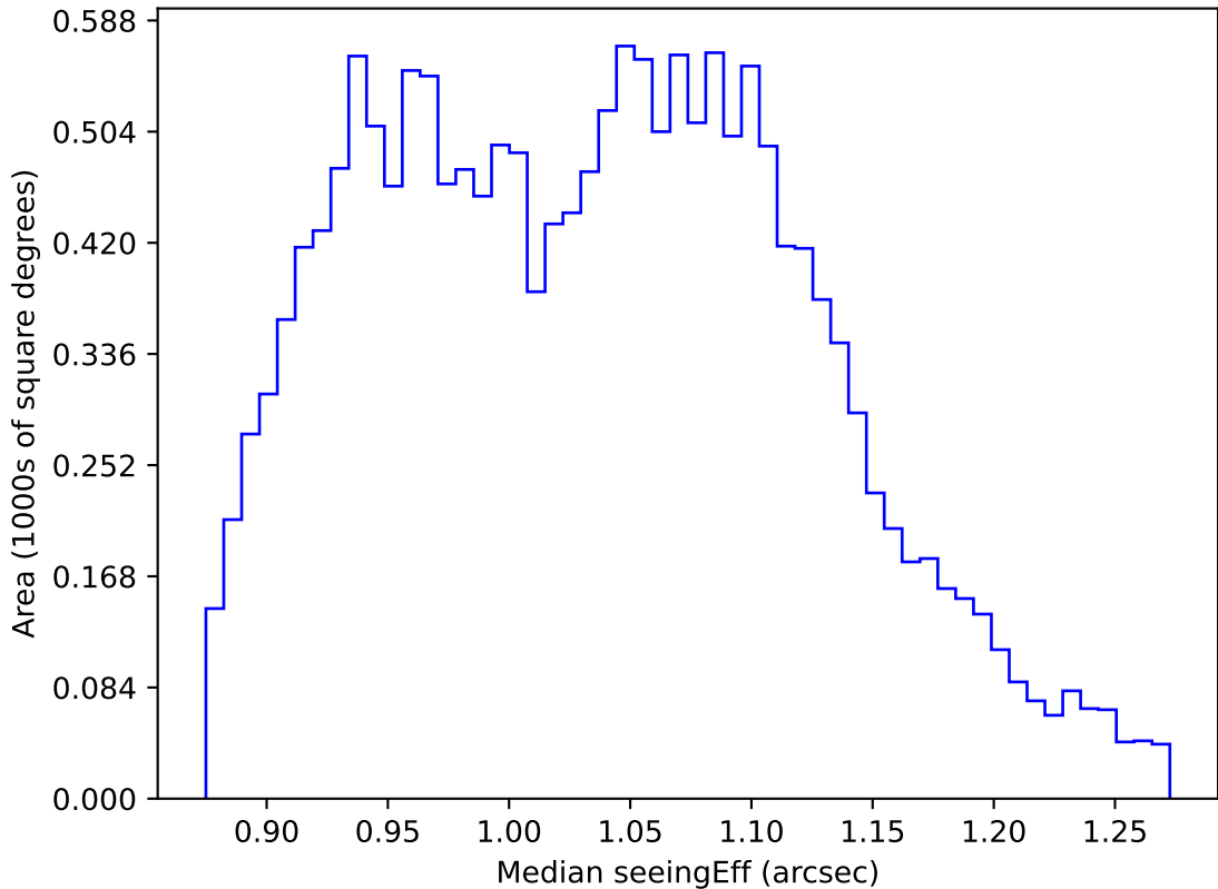
ddf_acor_sf30_lsf40_lsr20_v3.4_10yrs WFD r band: Median seeingEff
