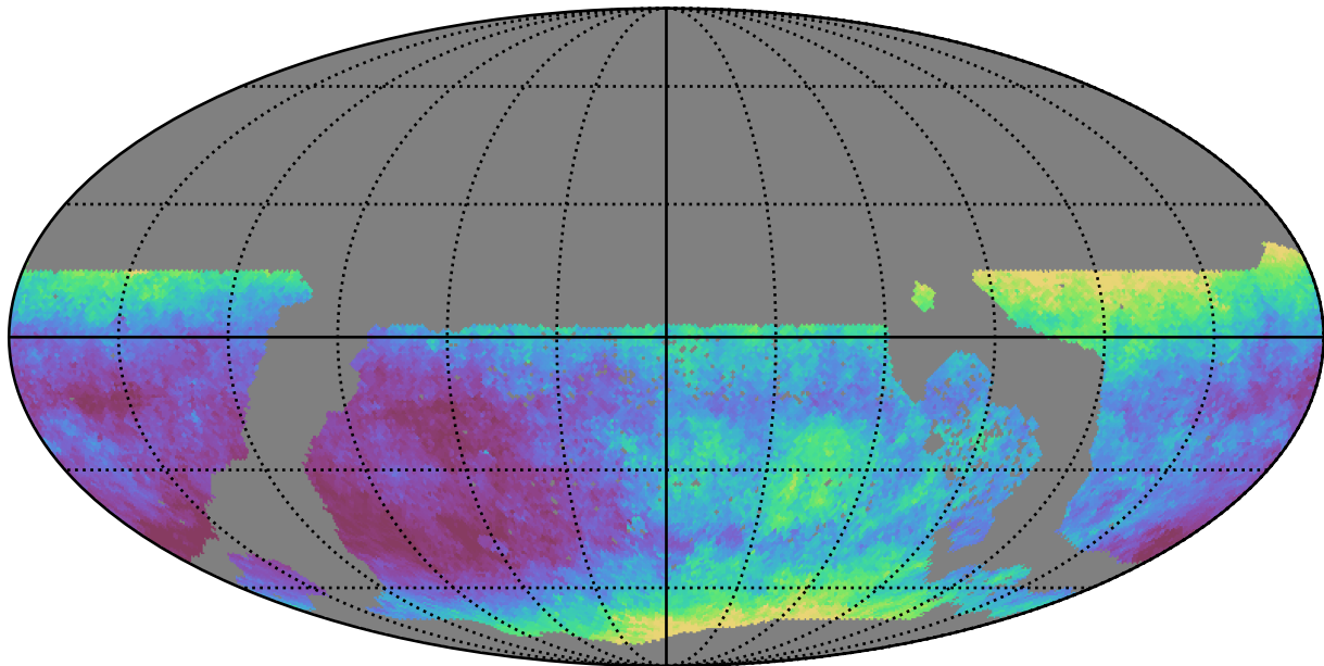
ddf_acor_sf30_lsf40_lsr20_v3.4_10yrs WFD i band: Median seeingEff
