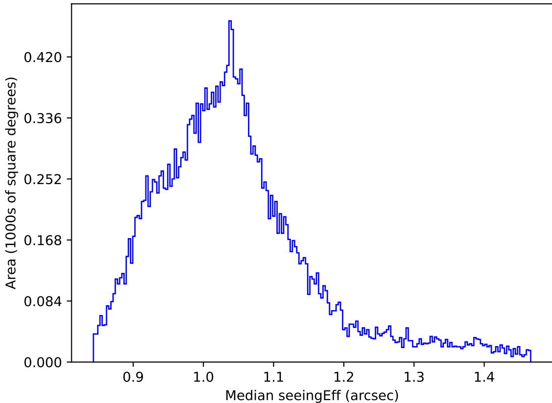
ddf_acor_sf30_ls40_lsr20_v3.4_10yrs All sky z band: Median seeingEff
