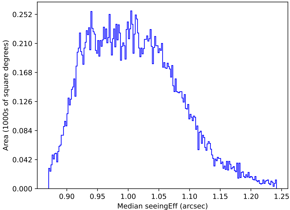
ddf_acor_sf30_ls40_lsr20_v3.4_10yrs All sky y band: Median seeingEff
