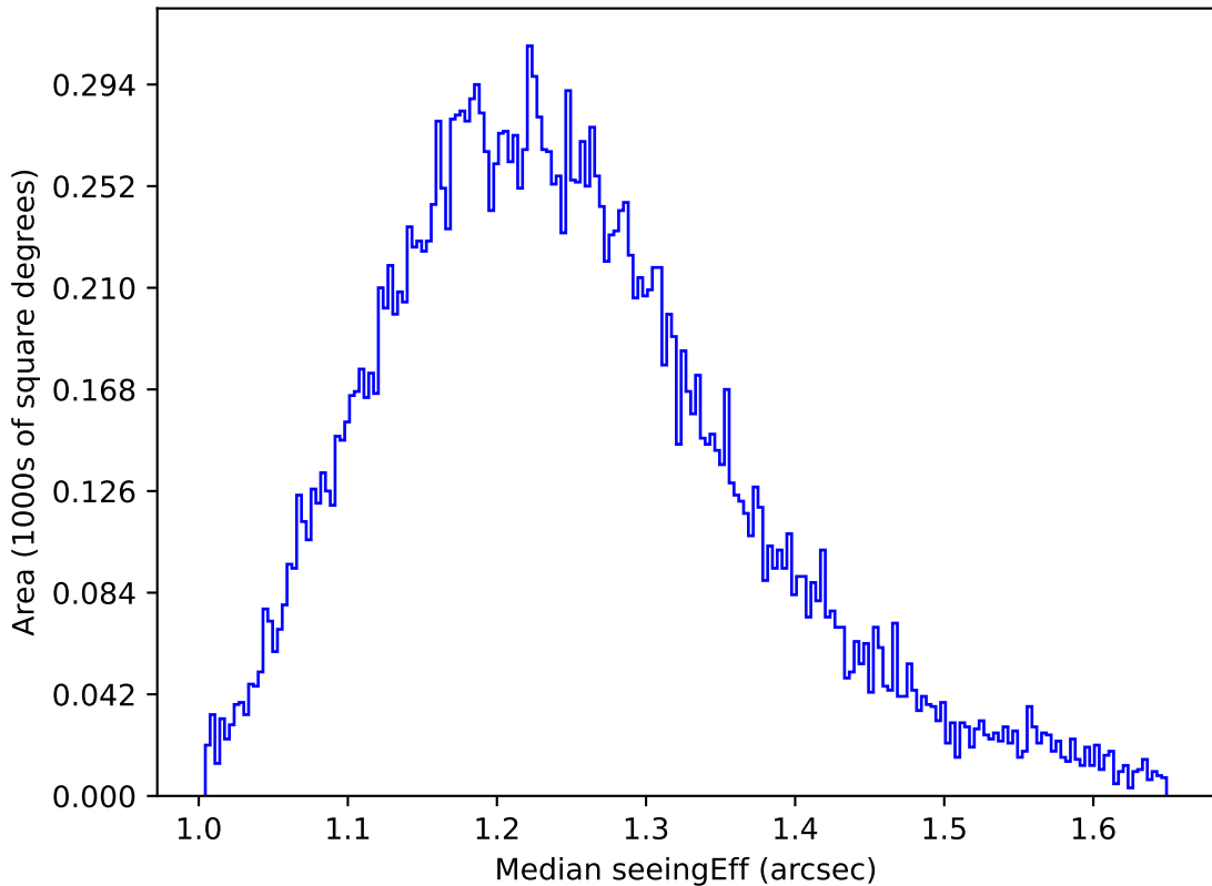
ddf_acor_sf30_ls40_lsr20_v3.4_10yrs All sky u band: Median seeingEff
