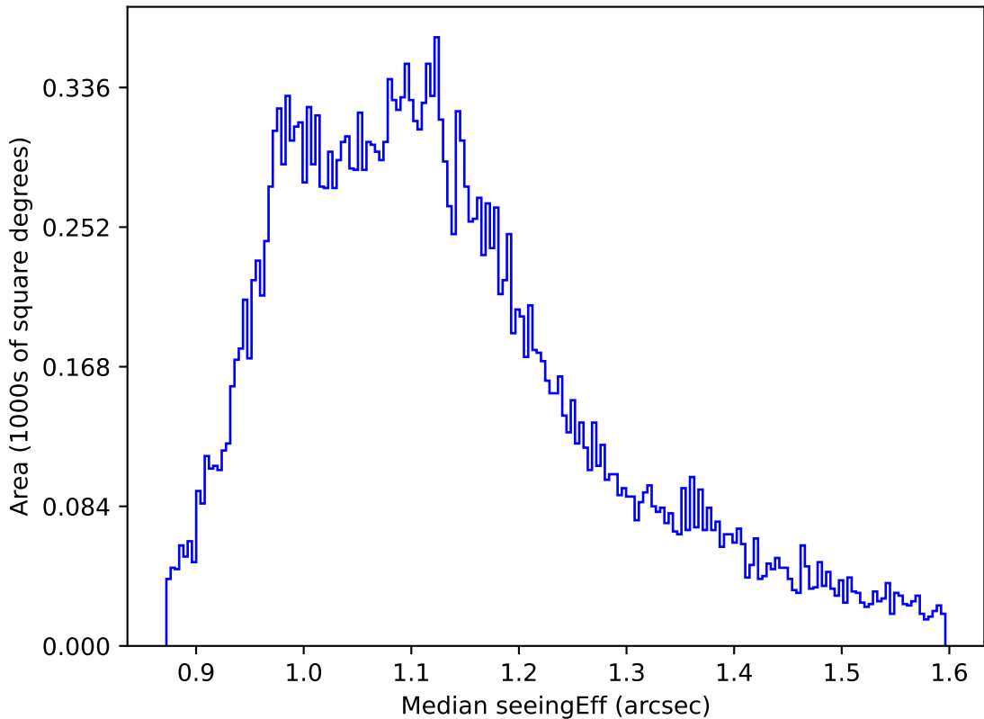
ddf_acor_sf30_lsf40_lsr20_v3.4_10yrs All sky g band: Median seeingEff
