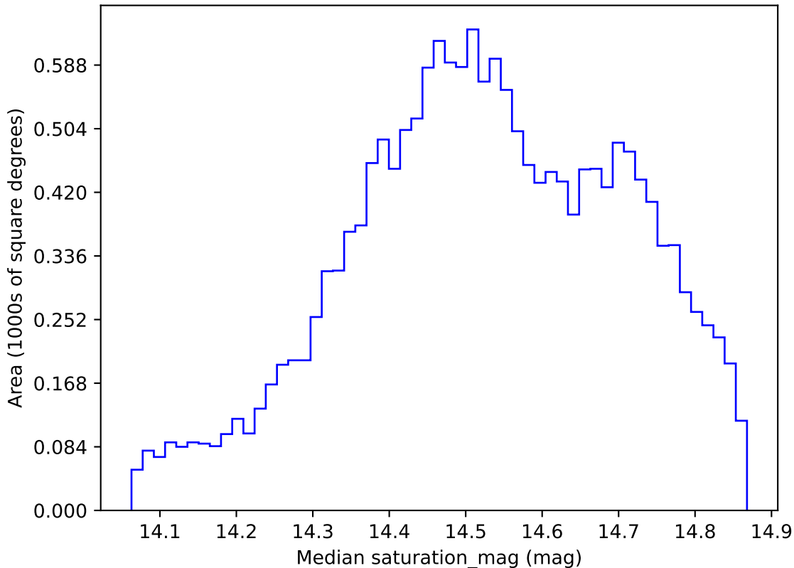
ddf_acor_sf30_lsf40_lsr20_v3.4_10yrs WFD i band: Median saturation_mag
