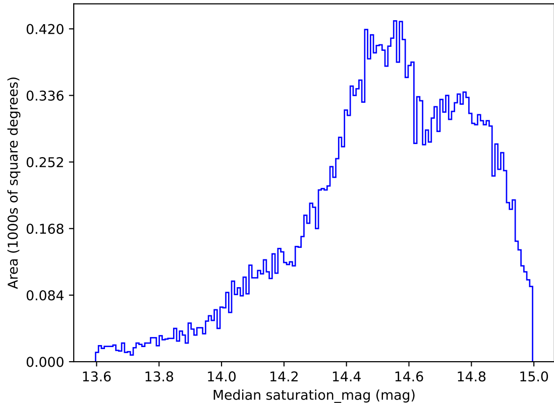
ddf_acor_sf30_lsf40_lsr20_v3.4_10yrs All sky r band: Median saturation_mag
