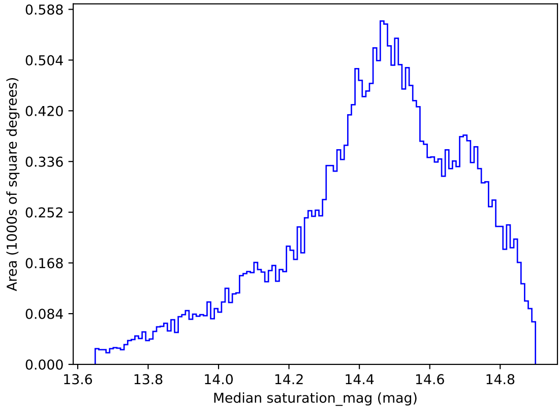
ddf_acor_sf30_lsf40_lsr20_v3.4_10yrs All sky i band: Median saturation_mag
