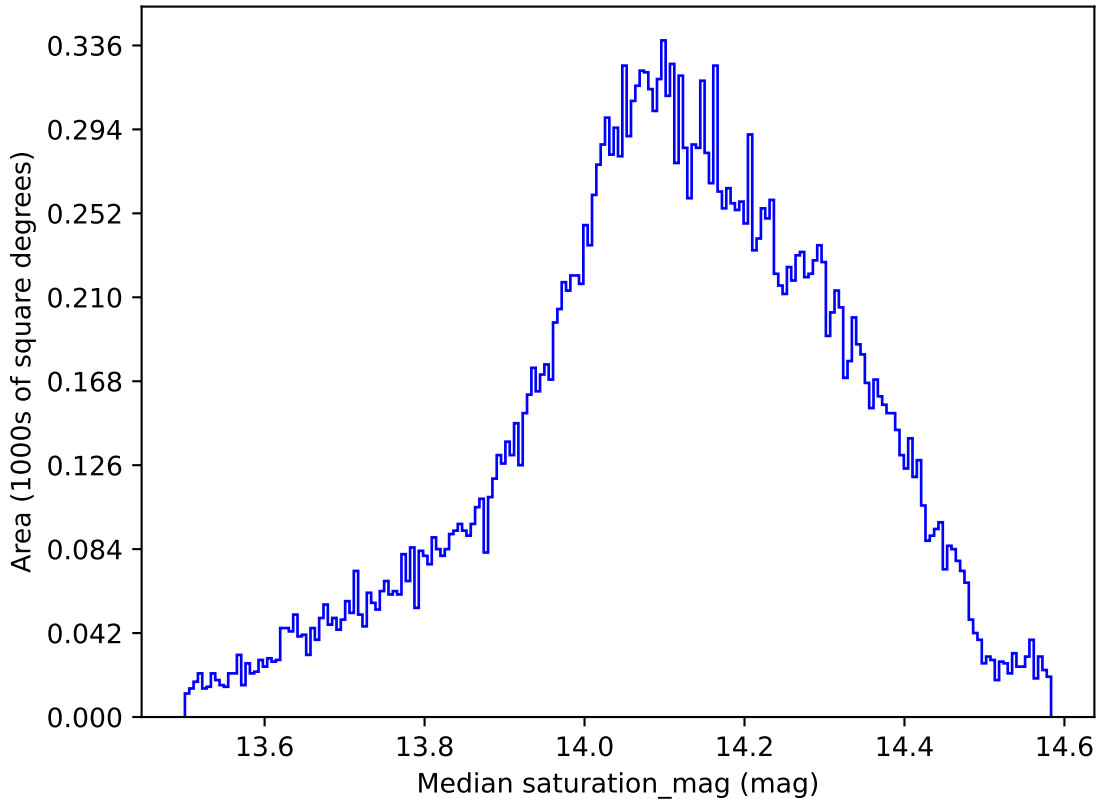
ddf_acor_sf30_lsf40_lsr20_v3.4_10yrs All sky all bands: Median saturation_mag
