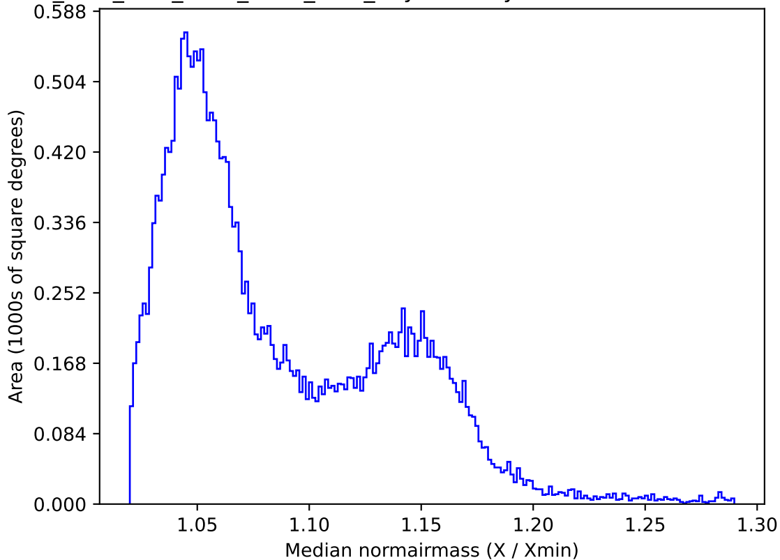
ddf_acor_sf30_lsf40_lsr20_v3.4_10yrs All sky z band: Median normairmass
