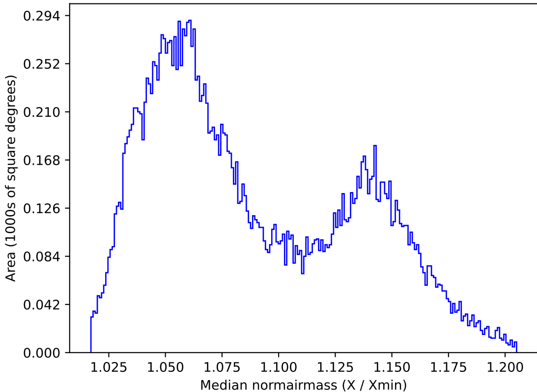
ddf_acor_sf30_ls40_lsr20_v3.4_10yrs All sky y band: Median normairmass
