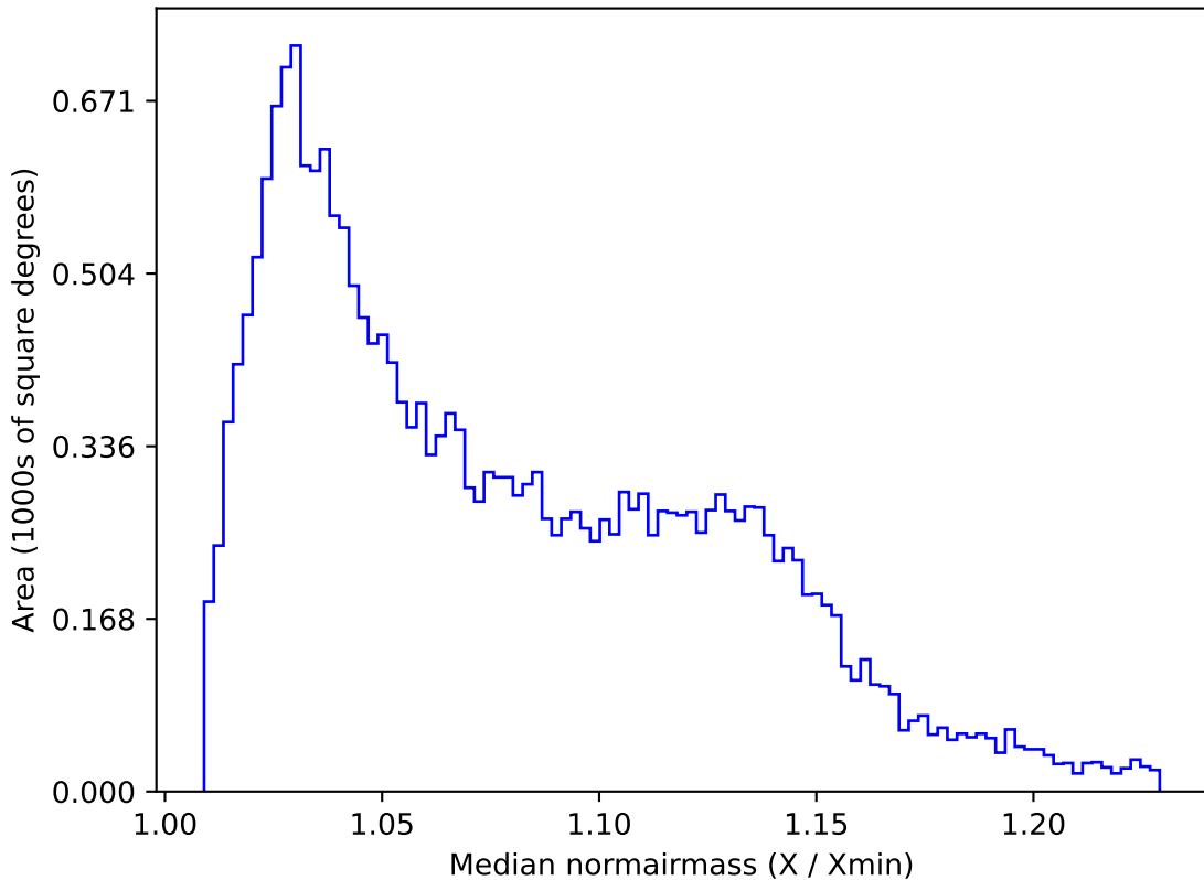
ddf_acor_sf30_lsf40_lsr20_v3.4_10yrs All sky u band: Median normairmass
