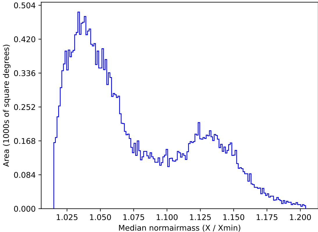
ddf_acor_sf30_lsf40_lsr20_v3.4_10yrs All sky r band: Median normairmass
