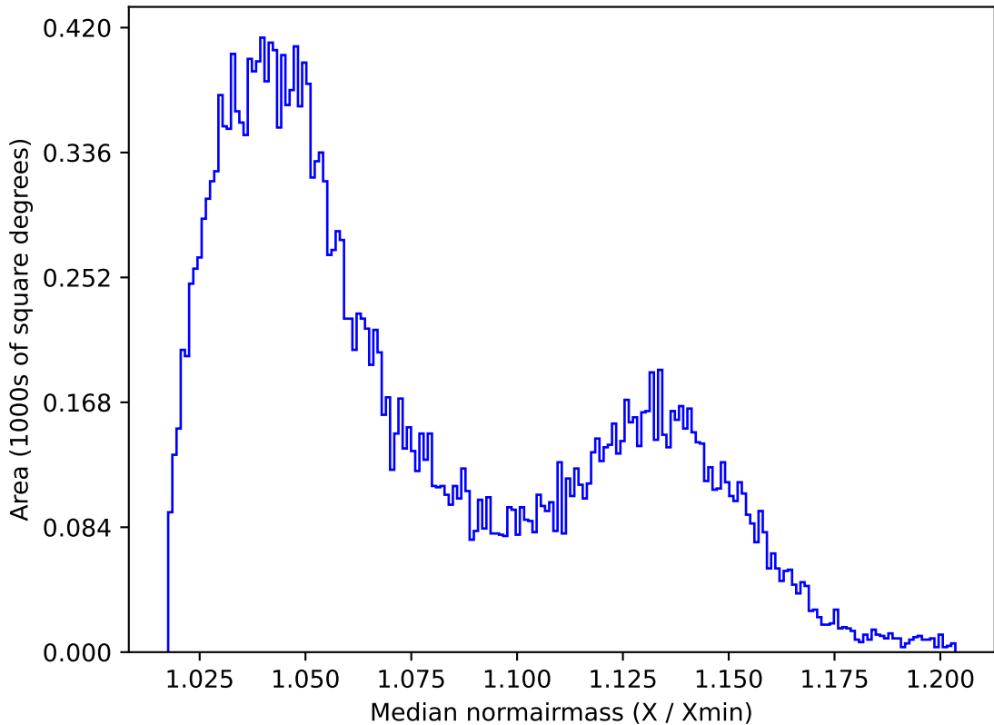
ddf_acor_sf30_lsf40_lsr20_v3.4_10yrs All sky i band: Median normairmass
