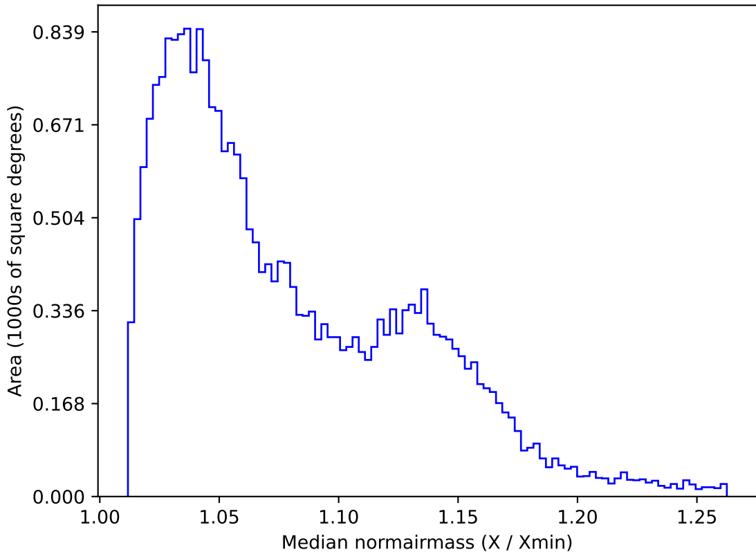
ddf_acor_sf30_lsf40_lsr20_v3.4_10yrs All sky g band: Median normairmass
