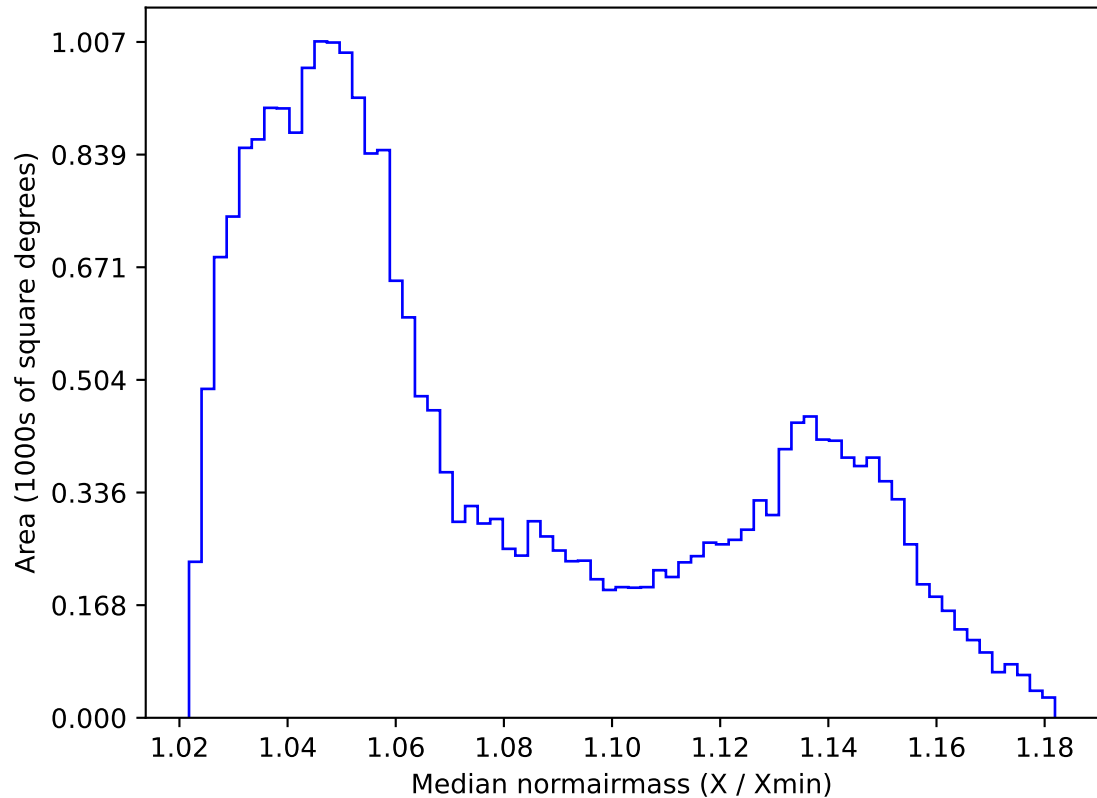
ddf_acor_sf30_lsf40_lsr20_v3.4_10yrs All sky all bands: Median normairmass
