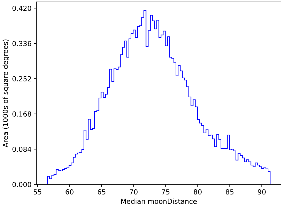
ddf_acor_sf30_lsf40_lsr20_v3.4_10yrs WFD z band: Median moonDistance
