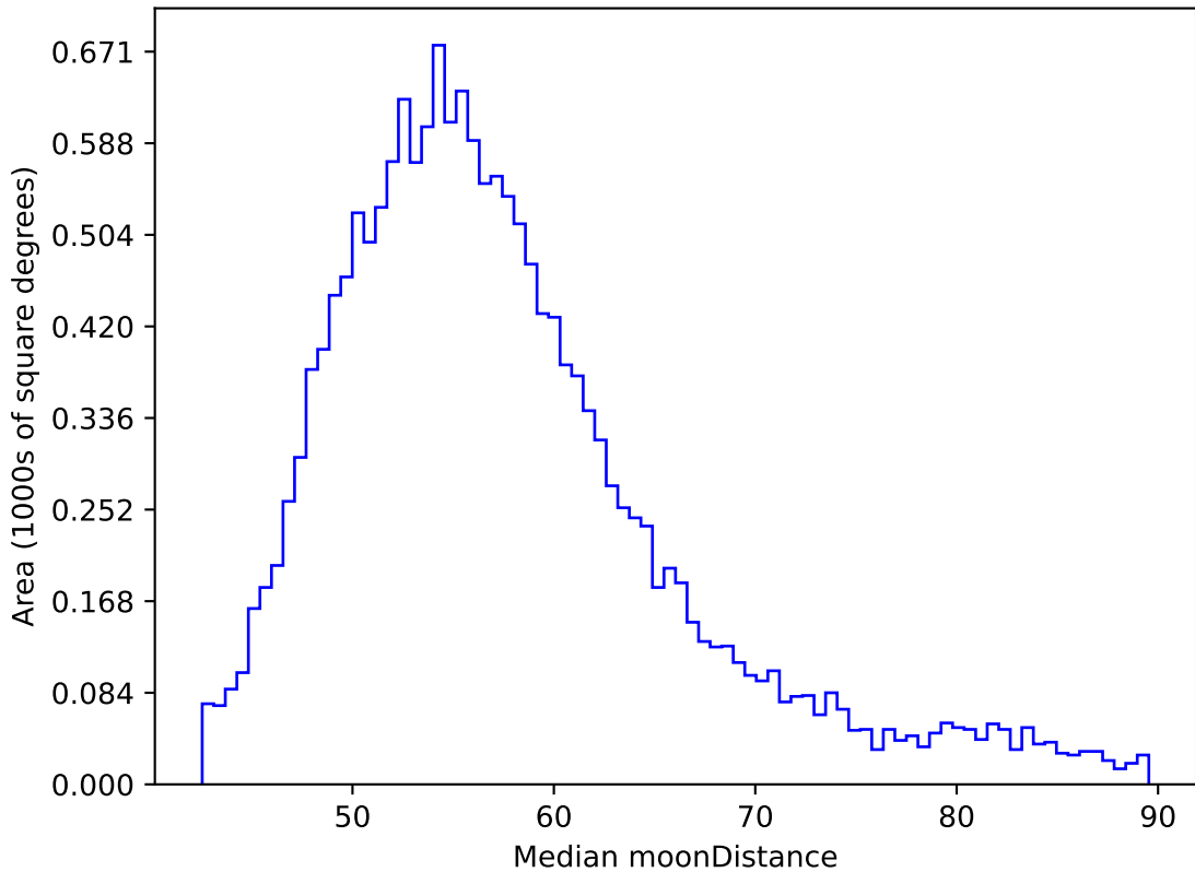
ddf_acor_sf30_lsf40_lsr20_v3.4_10yrs WFD y band: Median moonDistance
