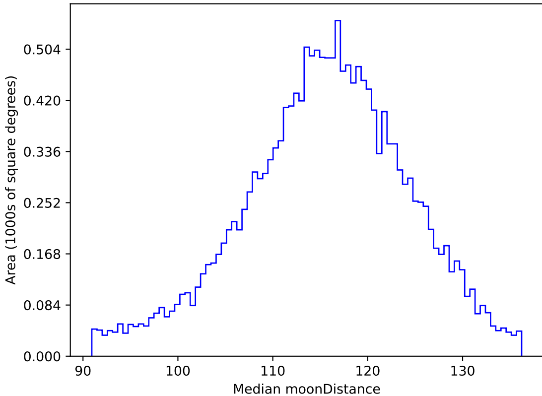
ddf_acor_sf30_lsf40_lsr20_v3.4_10yrs WFD g band: Median moonDistance
