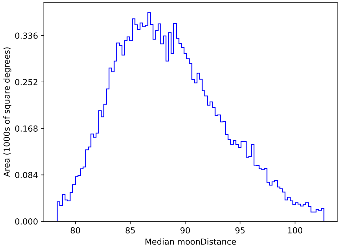
ddf_acor_sf30_lsf40_lsr20_v3.4_10yrs WFD all bands: Median moonDistance
