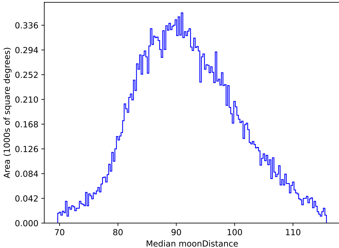
ddf_acor_sf30_lsf40_lsr20_v3.4_10yrs All sky i band: Median moonDistance
