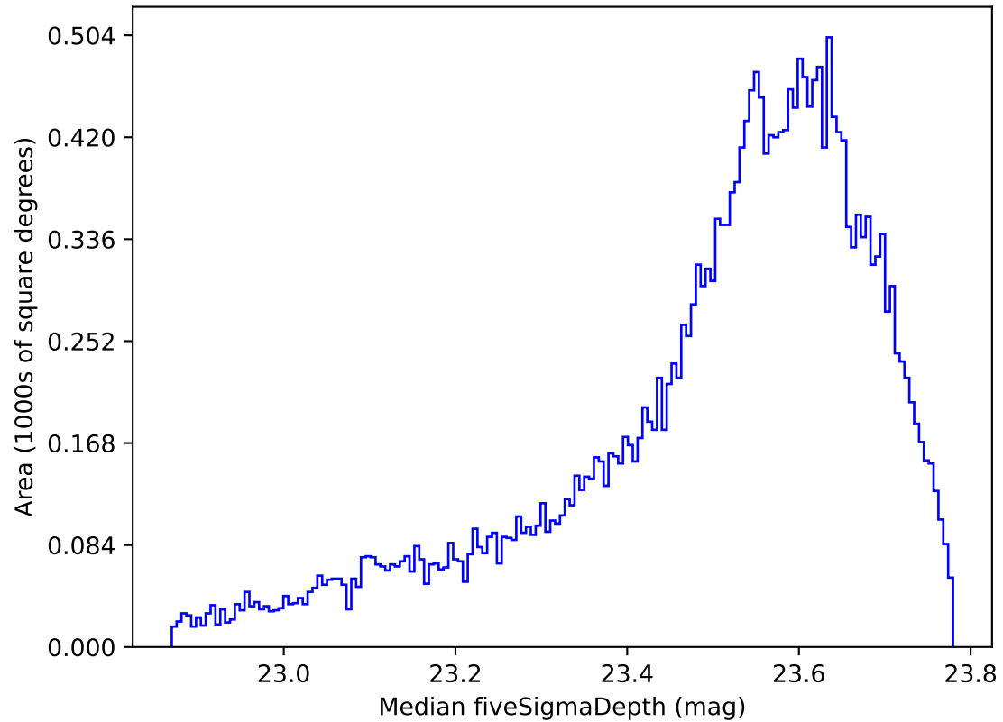
ddf_acor_sf30_lsf40_lsr20_v3.4_10yrs All sky i band: Median fiveSigmaDepth
