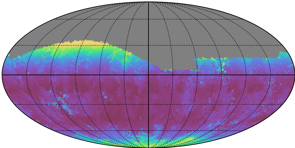
ddf_acor_sf30_lsf40_lsr20_v3.4_10yrs Yr 1 g band: Median airmass
