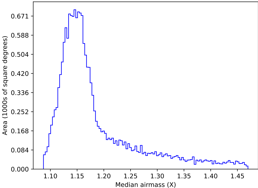
ddf_acor_sf30_lsf40_lsr20_v3.4_10yrs WFD z band: Median airmass
