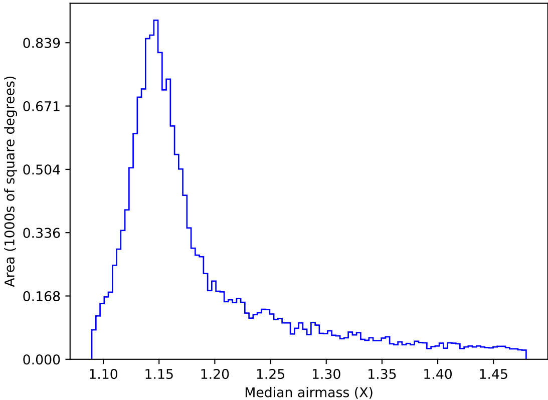
ddf_acor_sf30_lsf40_lsr20_v3.4_10yrs WFD y band: Median airmass
