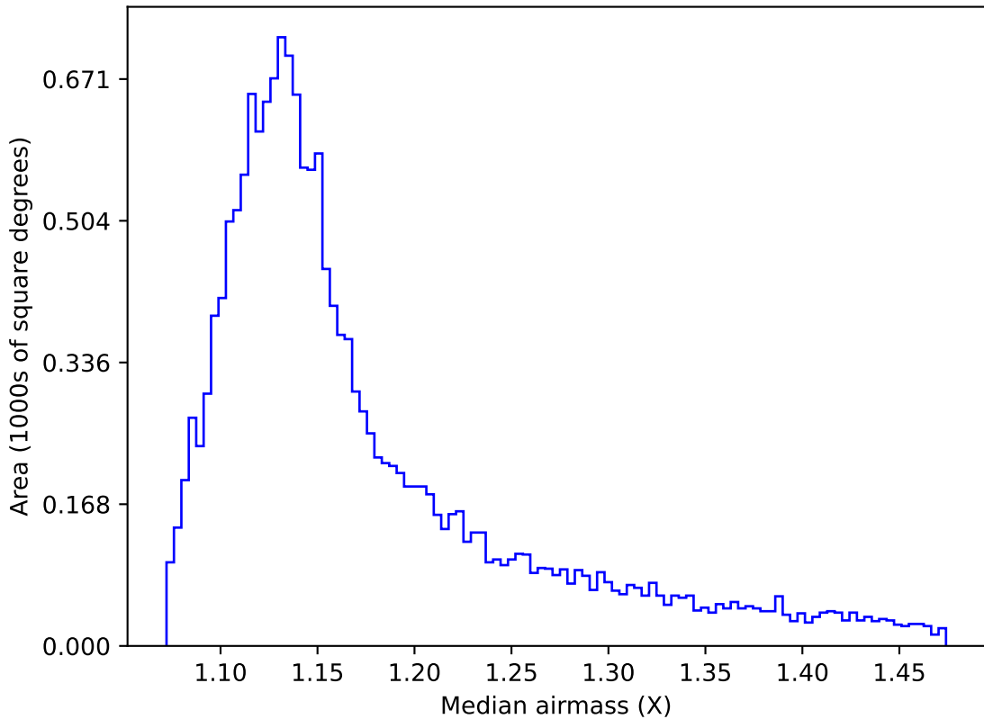
ddf_acor_sf30_lsf40_lsr20_v3.4_10yrs WFD u band: Median airmass
