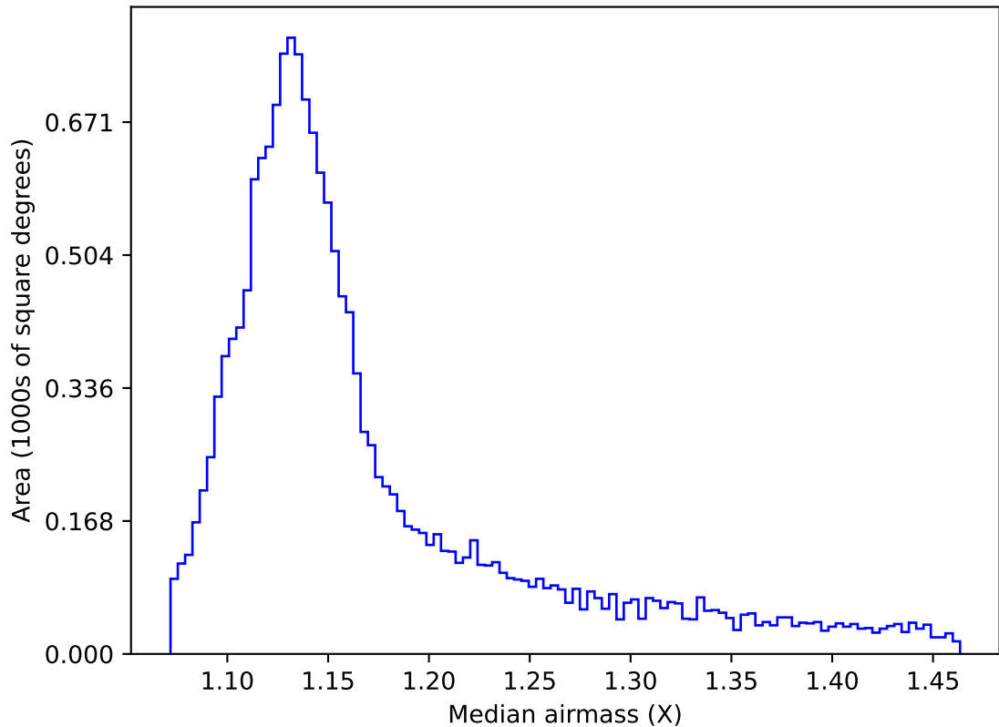
ddf_acor_sf30_lsf40_lsr20_v3.4_10yrs WFD r band: Median airmass
