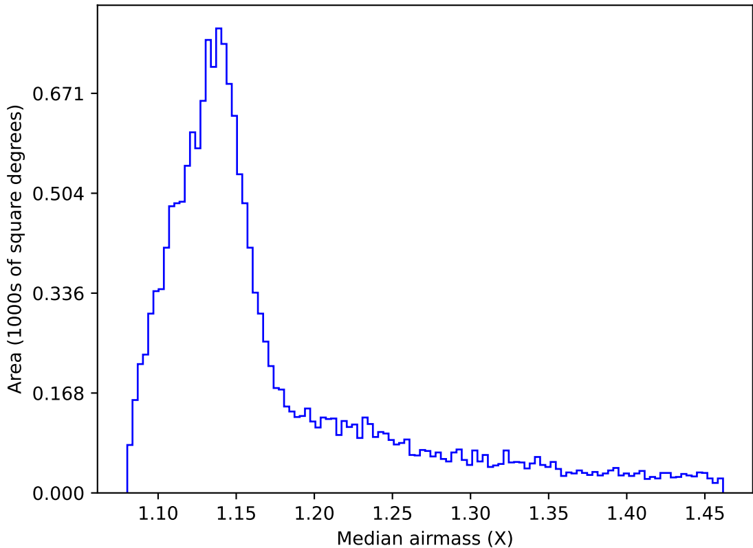
ddf_acor_sf30_lsf40_lsr20_v3.4_10yrs WFD i band: Median airmass
